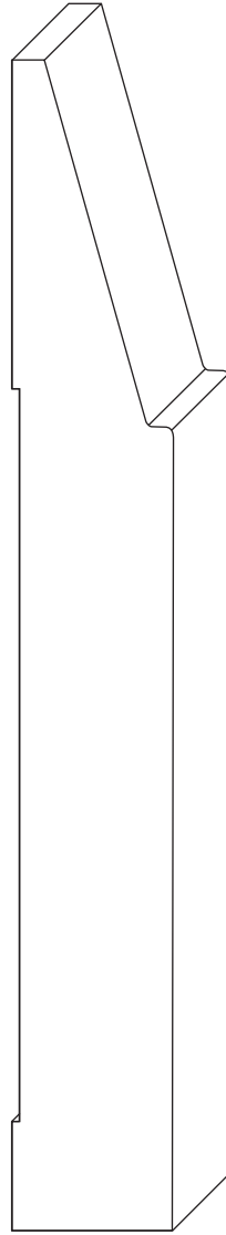
5-1/2" CONTEMPORARY BASEBOARD AK#518 ●
