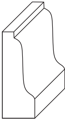
PANEL MOULD #189 ● ▲
