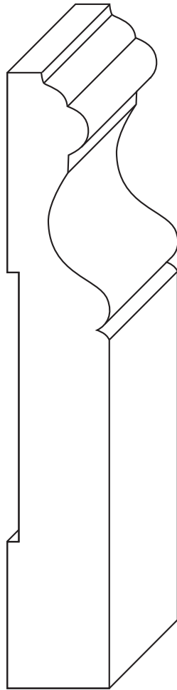
4 1/2" COLONIAL BASEBOARD AK#88 ● ▲ ■ ◆
