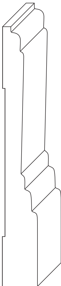
5 1/2" HOPPER BASEBOARD ●
